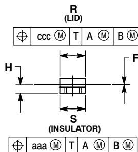
CASE 360B-05 ISSUE F NI-360 MRF9030LR1
